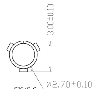
SEC:C-C
